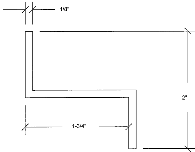
FRP Z ASTRAGAL
